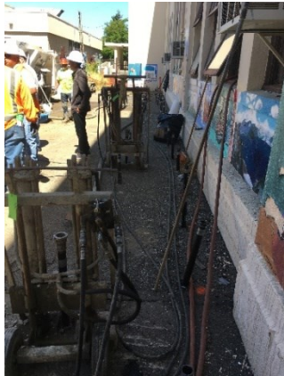
Grout injection, Exterior
